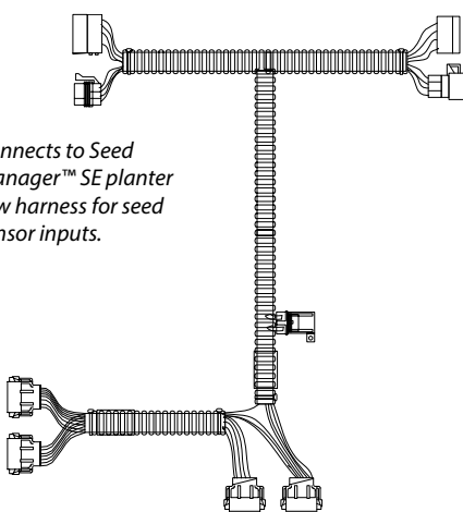
WSMB Harness SE Style 467981201A
